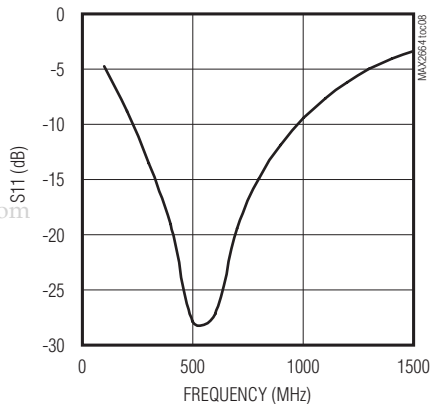
MAX2664 S11 BYPASS MODE
