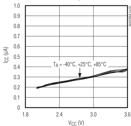
MAX2664/MAX2665 I_{CC} vs. V_{CC} BYPASS MODE, CTRL = GND
