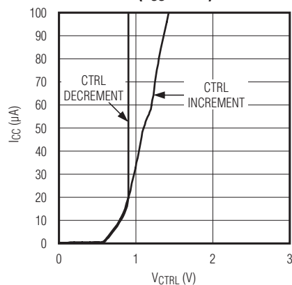
MAX2664/MAX2665 I_{CC} vs. V_{CTRL} ( V_{CC} = 2.7V )
