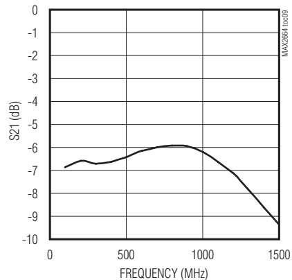
MAX2664 S21 BYPASS MODE
