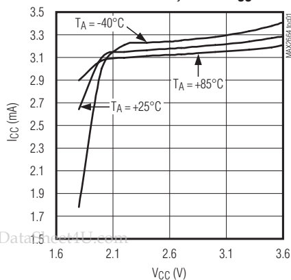
MAX2664/MAX2665 I_{CC} vs. V_{CC} NORMAL MODE, CTRL = V_{CC}
